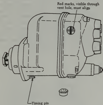
FIGURE 4-36. Checking magneto E-gap.
